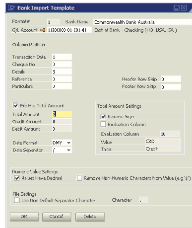
Bank Import Template Setup
